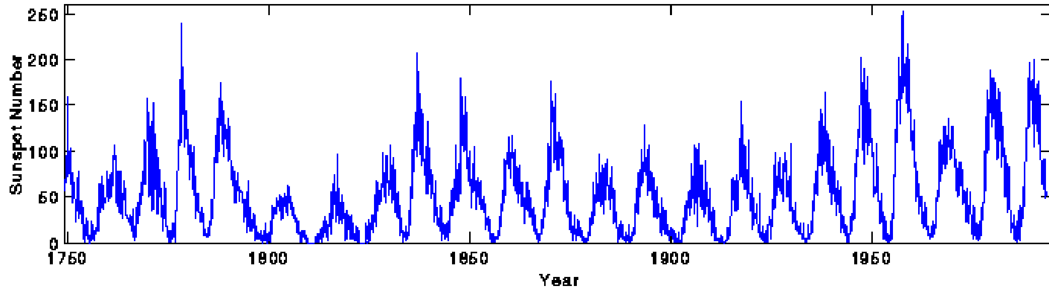
Sunspot Cycles from 1749 to Today
