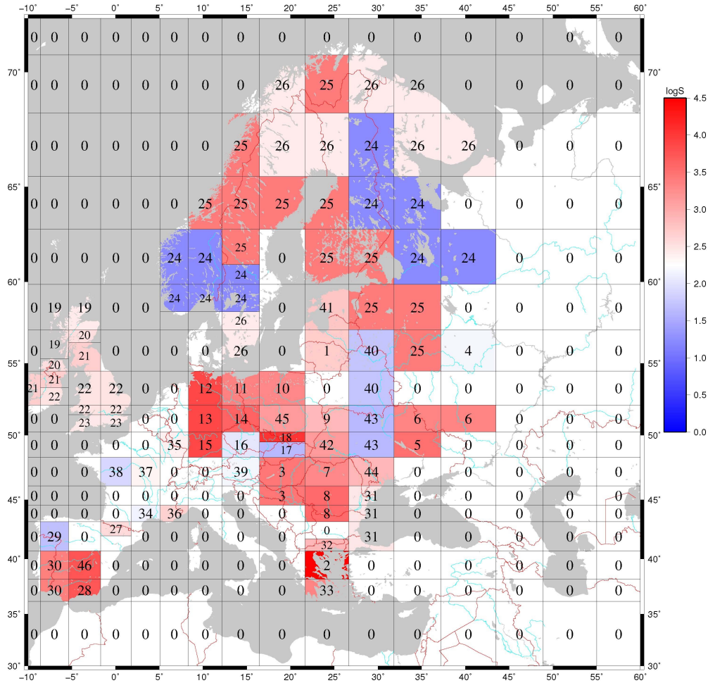
Conductance map of Europe (80 km)
