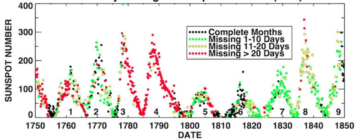
Monthly Averaged Sunspot Numbers (V2.0)
